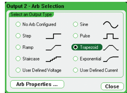
Figure 8. The Arb Selection menu is used to select which pre-programmed waveform will be applied to the output of the DC power module. Each of the four outputs can have a different waveform applied.
