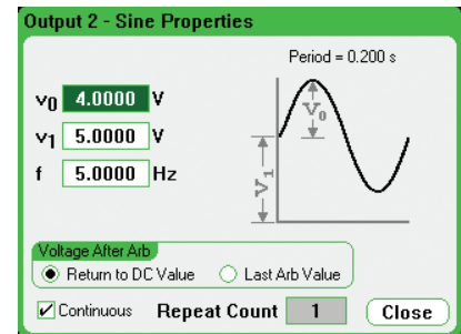
Figure 9. Once you have selected a waveform, you simply fill in the blanks to describe the waveform.
