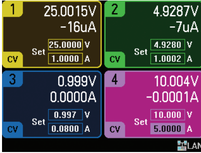
Figure 3. In Meter View, all 4 outputs can be viewed simultaneously. The both measured values for voltage and current and setting for voltage and current are displayed for each output.
