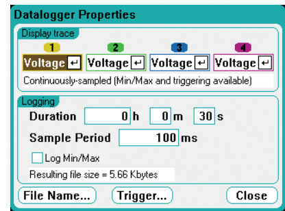
Figure 7. To set up the data logger, use a menu screen to select the operating parameters. Setup screens like this are used throughout the DC power analyzer.
